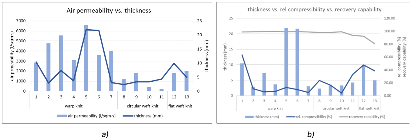
Figure 1. Air permeability vs. thickness and thickness vs. compressibility vs. recovery, x-axis: samples by knitting technology.
