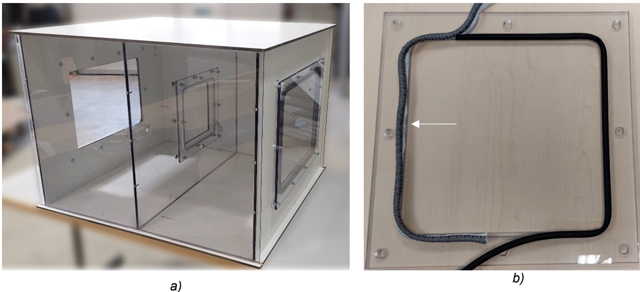
Figure 2 a) Basic construction of the two-chamber test bench. The two plates on the front sides with the cut-outs are placeholders for the technical plates with measurement equipment and e.g. fans to introduce air pressure; b) For illustrative purposes the recess in the partition wall was sealed with a textile prototype (white arrow) inside a standard window groove.
