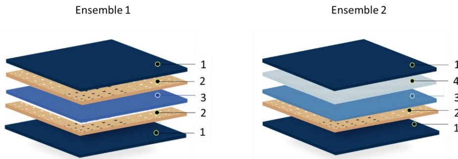
Fig. 1 Proposed ensembles for vest architecture: 1) outer shell fabric; 2) microperforated material composed by biologically degradable insulating cellulose cells; 3) PCM pouches layer; 4) 3D knitted fabric.
