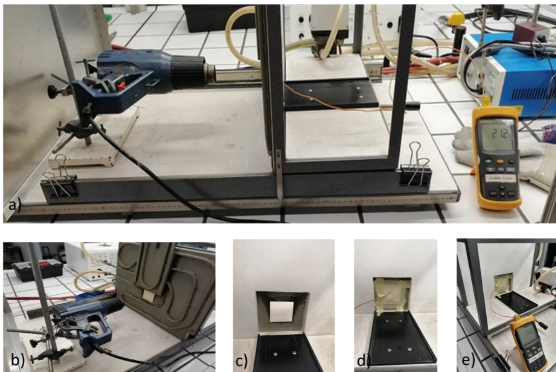
Fig. 3 Experimental set-up for preliminary evaluation of PCM pouches: a) global view; b) heat source; c) sample frame; d) sample placed in the frame connected to a thermocouple; e) temperature acquisition device.
