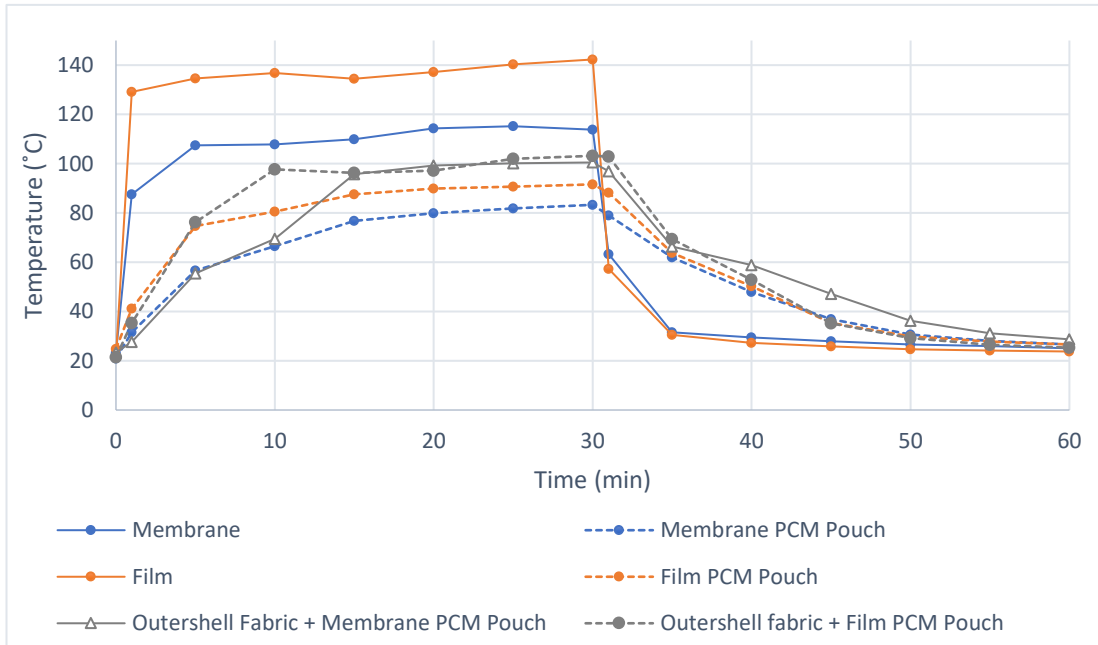
Fig. 8 Thermal performance of the materials used in the vest with PCM integration.
