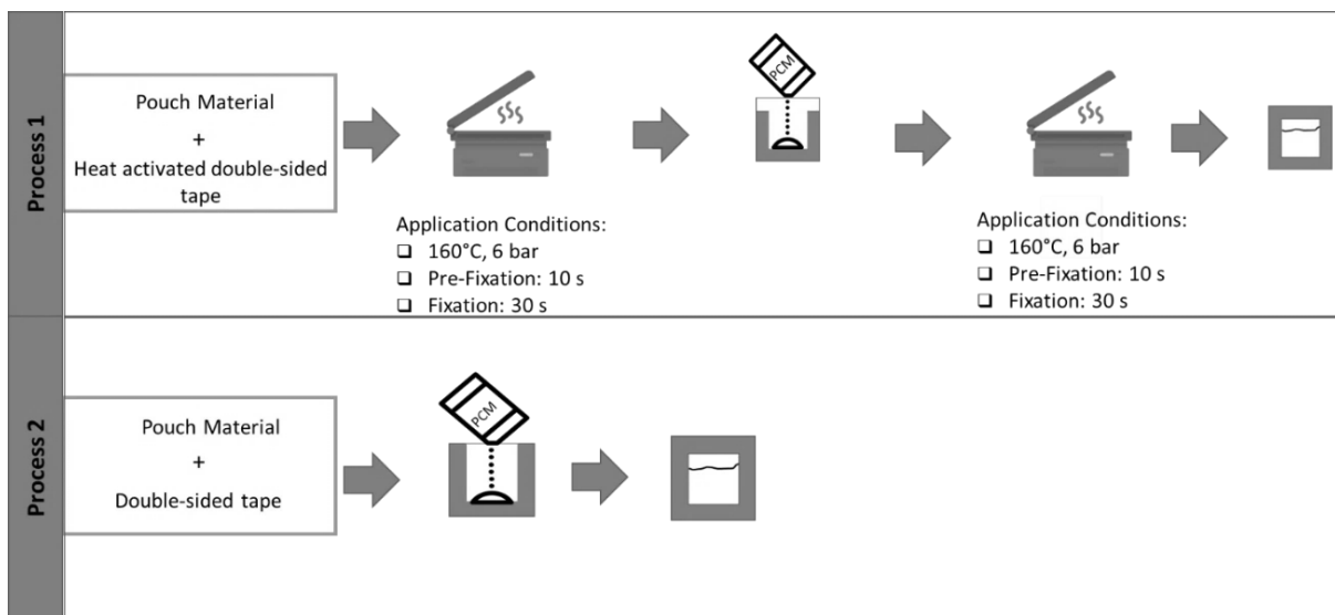
Fig. 2 Different processes used for PCM pouches development using bonding technology.
