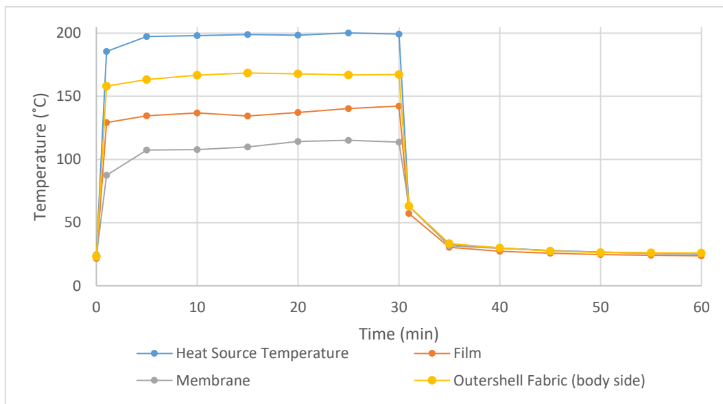
Fig. 7 Thermal performance of the materials used in the vest without PCM integration.
