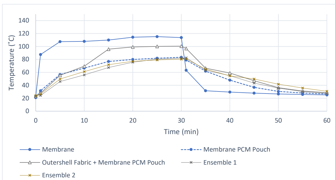
Fig. 9 Thermal performance evaluation of the two ensembles proposed.
